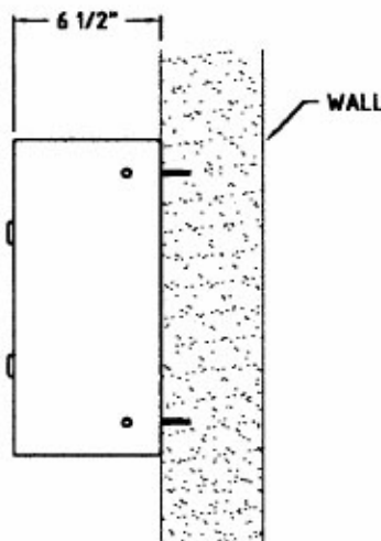
SURFACE MOUNT HGS
